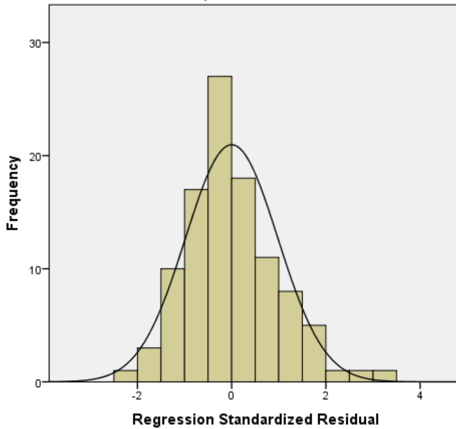
Histogram of Standardized Residuals
